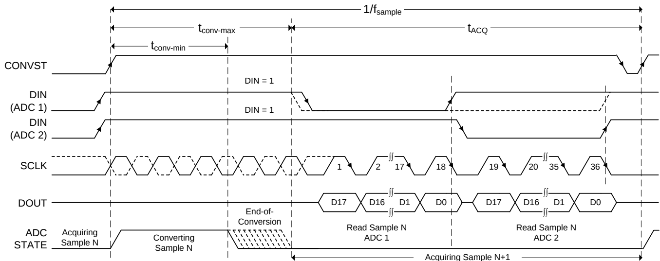
Figure 49. Interface Timing Diagram: Two ADCs with 4-Wire \overline{CS} Mode
