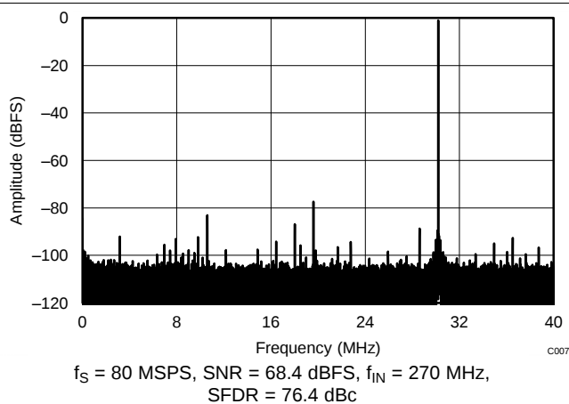
Figure 73. FFT for 270-MHz Input Signal (Dither On)
