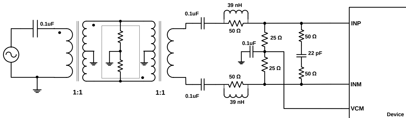
Figure 22. Driving Circuit for Low Input Frequencies
