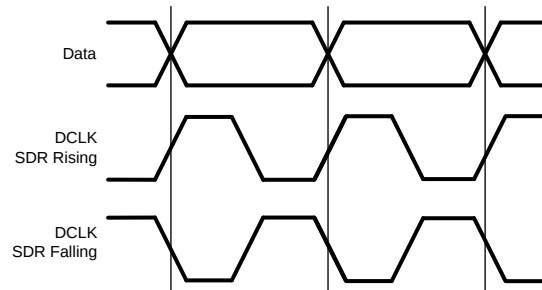
Figure 41. SDR DCLK-to-Data Phase Relationship
