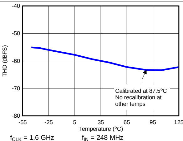
Figure 33. THD vs Temperature Calibration at 87.5°C Only
