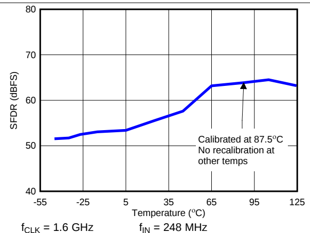
Figure 34. SFDR vs Temperature Calibration at 87.5°C Only
