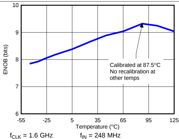
Figure 31. ENOB vs Temperature Calibration at 87.5°C Only
