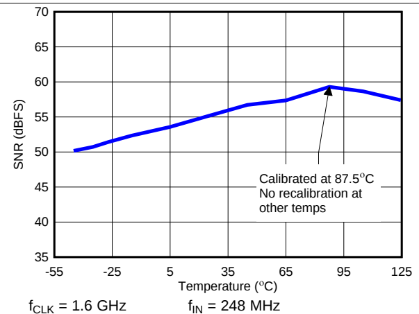
Figure 32. SNR vs Temperature Calibration at 87.5°C Only
