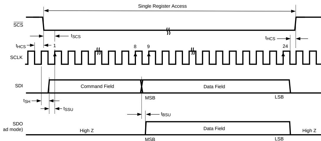
Figure 9. Serial Interface Timing
