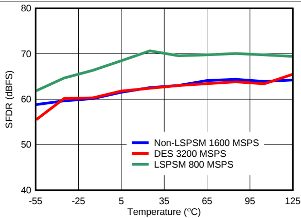
Figure 29. SFDR vs Temperature
