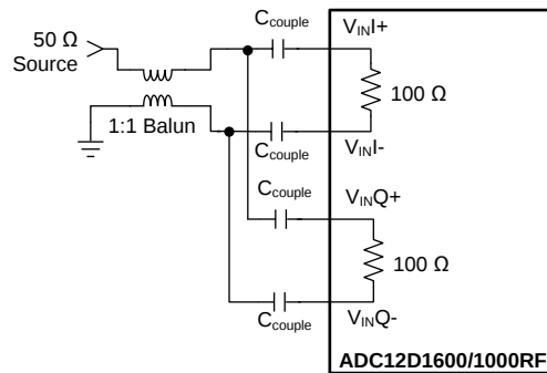
Figure 44. Driving DESIQ Mode
