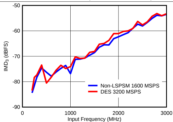
Figure 35. 3rd Order Intermodulation Distortion vs Input Frequency
