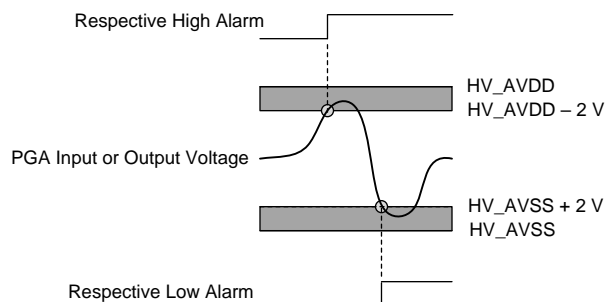
Figure 31. PGA Monitor Thresholds
