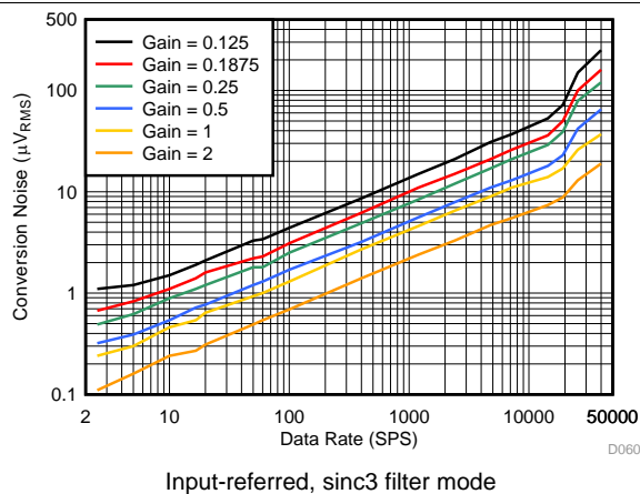
Figure 10. Noise ( e_n ) vs Data Rate, Gain = 0.125 to 2
