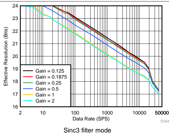
Figure 6. Effective Resolution vs Data Rate, Gain = 0.125 to 2
