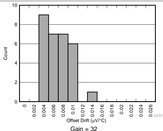
Figure 19. Offset Error Drift Distribution Histogram
