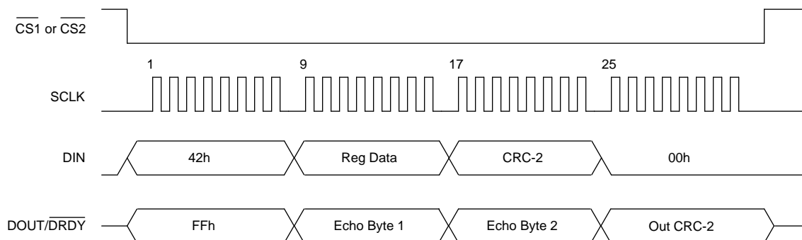
Figure 47. Register Write Command Sequence (Address = 02h)
