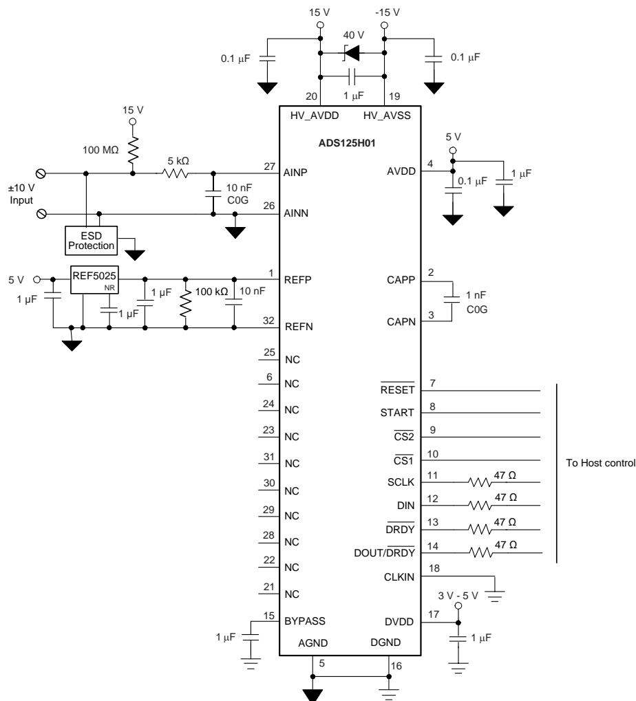
Figure 64. \pm 10 -V Analog Input PLC Module
