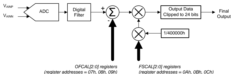
Figure 45. Calibration Block Diagram
