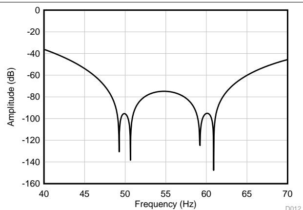
Figure 43. FIR Filter Frequency Response (20 SPS)
