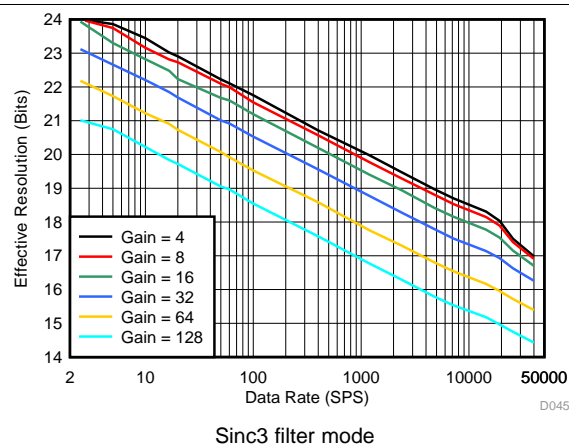
Figure 7. Effective Resolution vs Data Rate, Gain = 4 to 128
