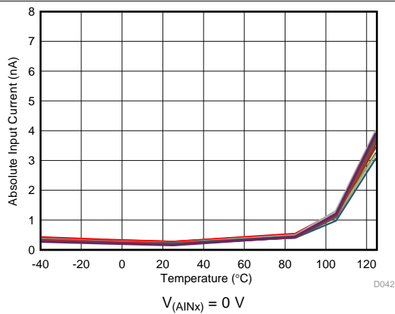
Figure 12. Absolute Analog Input Current vs Temperature
