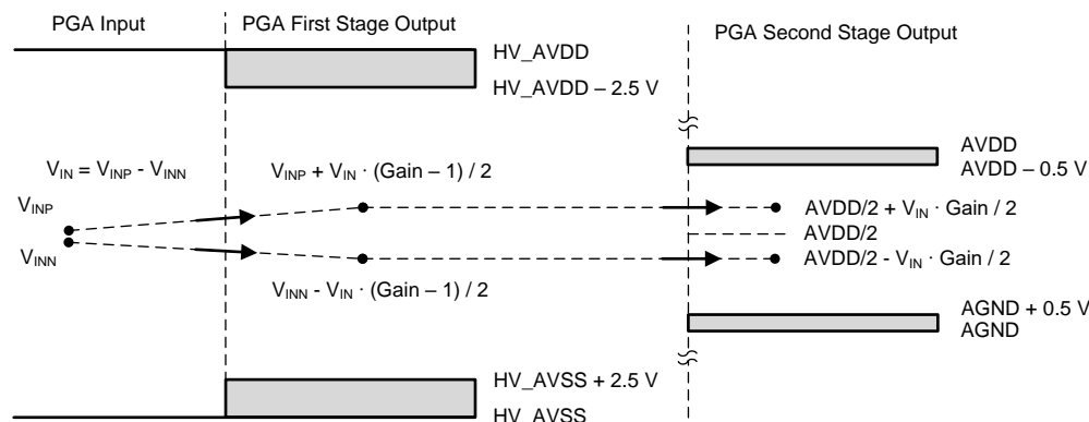
Figure 30. PGA Gain Mode
