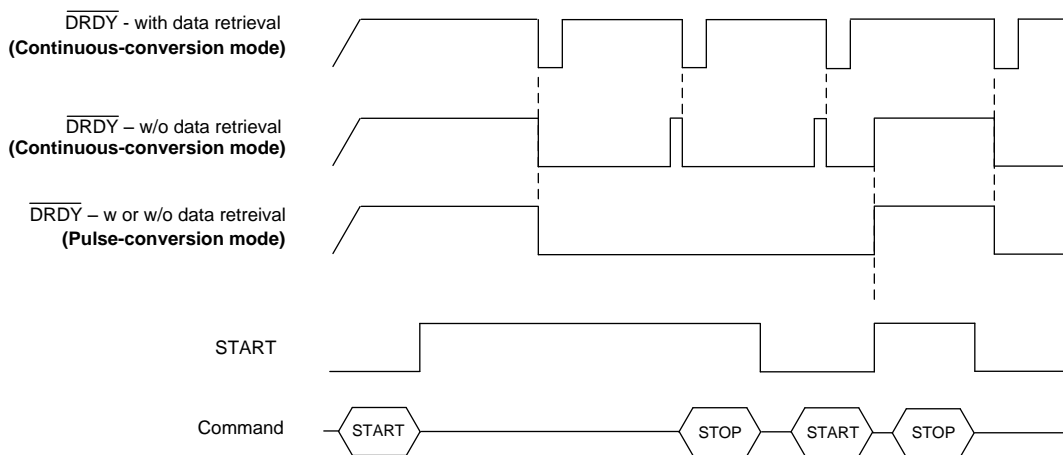
Figure 46. \overline{DRDY} Operation
