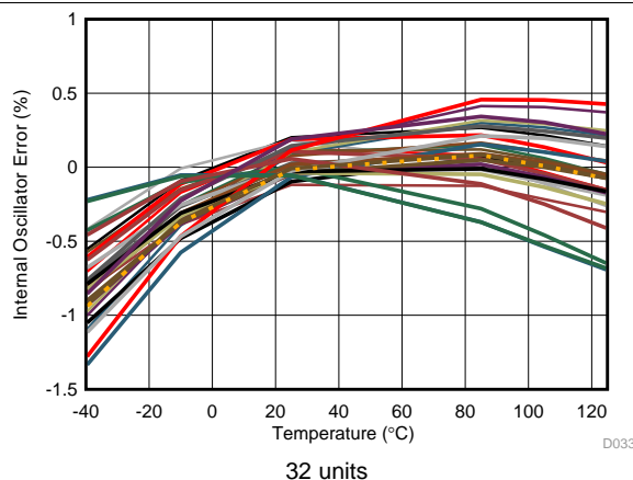
Figure 23. Oscillator Frequency Error vs Temperature
