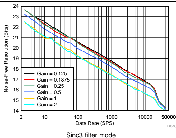
Figure 8. Noise-Free Resolution vs Data Rate, Gain = 0.125 to 2
