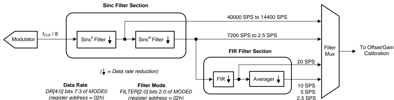
Figure 33. Digital Filter Block Diagram
