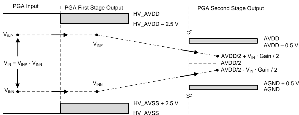
Figure 29. PGA Attenuation Mode
