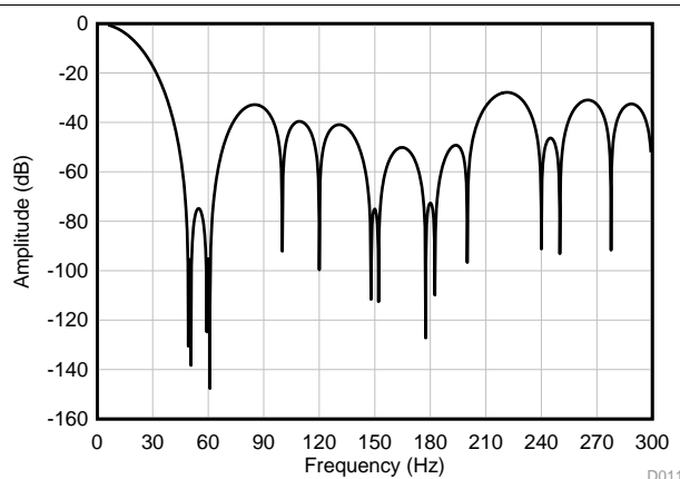
Figure 42. FIR Filter Frequency Response (20 SPS)
