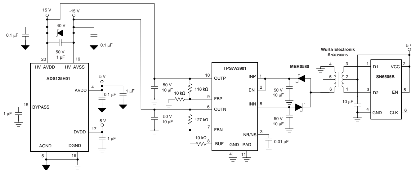
Figure 66. 5-V to \pm 15 -V DC/DC Converter
