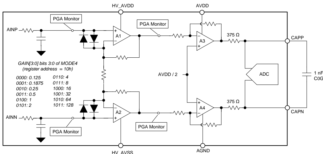
Figure 28. PGA Block Diagram
