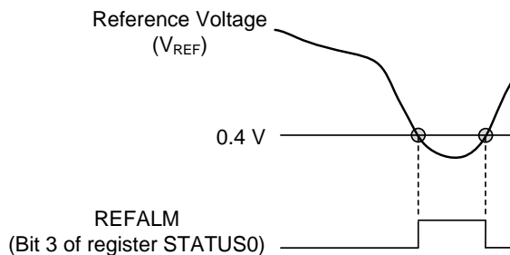
Figure 32. Reference Monitor Threshold
