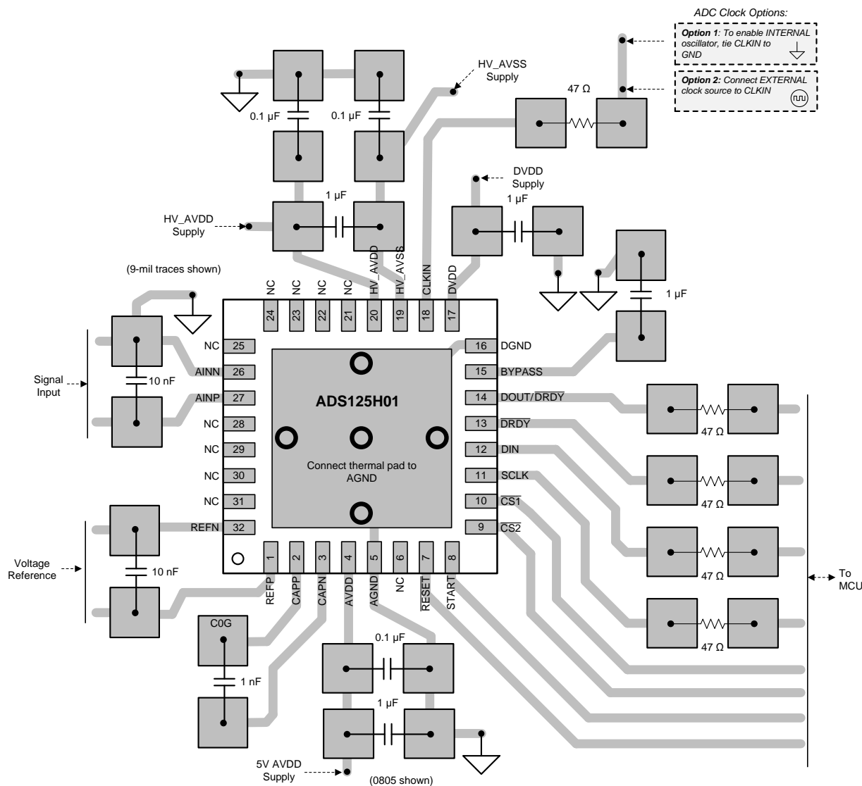
Figure 67. PCB Layout Example
