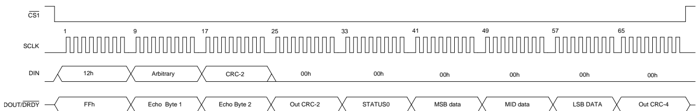
Figure 48. Conversion Data Read Operation
