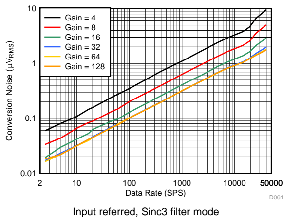
Figure 11. Noise ( e_n ) vs Data Rate, Gain = 4 to 128
