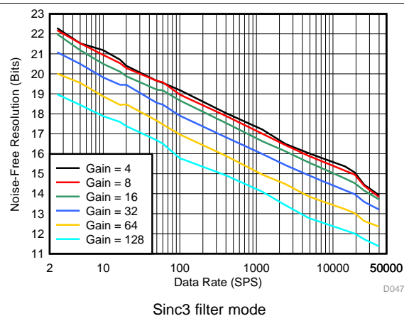
Figure 9. Noise-Free Resolution vs Data Rate, Gain = 4 to 128
