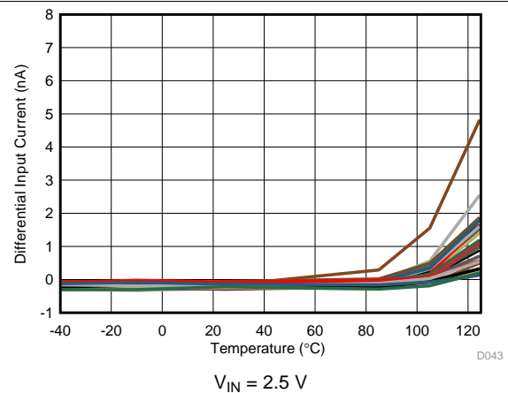
Figure 13. Differential Analog Input Current vs Temperature
