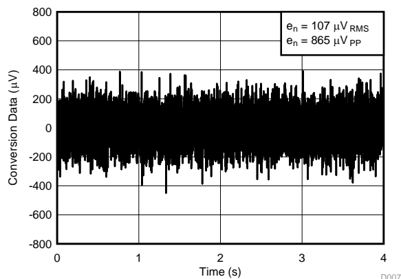
Figure 65. Conversion Noise
