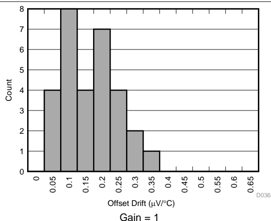
Figure 18. Offset Error Drift Distribution Histogram
