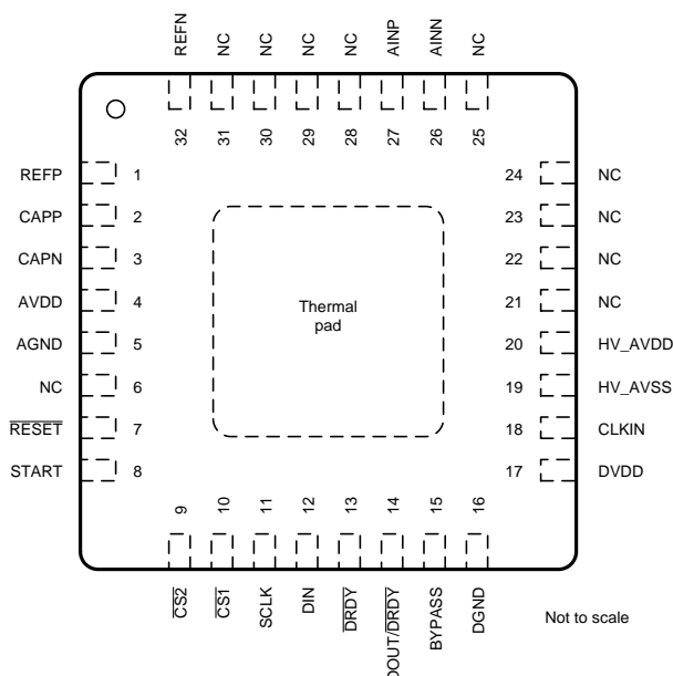
RHB Package 32-Pin VQFN Top View
