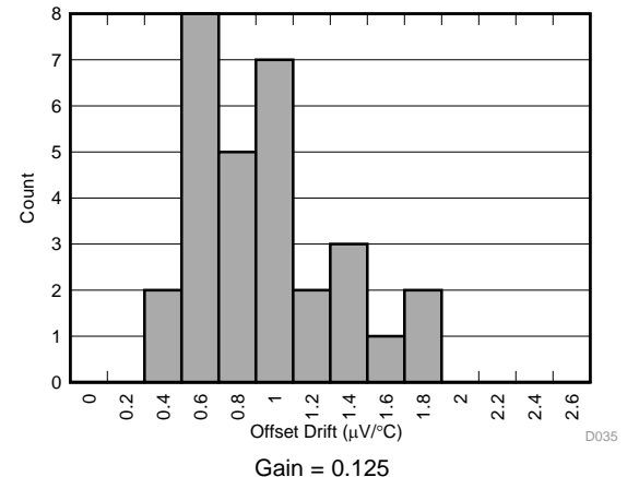
Figure 17. Offset Error Drift Distribution Histogram
