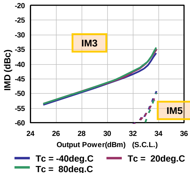
IMD vs. Output Power by Temperature
