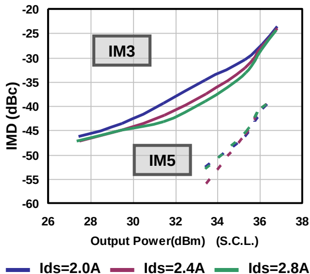
IMD v.s. Output Power by Quiescent Drain Current V_{DS}(DC)=10V@7.9GHz
