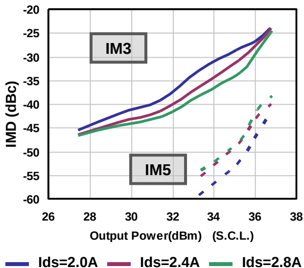
IMD v.s. Output Power by Quiescent Drain Current V_{DS}(DC)=10V@7.1GHz
