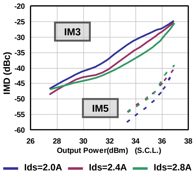
IMD v.s. Output Power by Quiescent Drain Current V_{DS}(DC)=10V@7.5GHz
