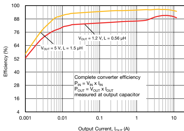
Fig. 10 - SiC437 Efficiency vs. Output Current (V_{IN} = 12\text{ V}, f_{SW} = 500\text{ kHz}, \text{Power Saving Mode})
