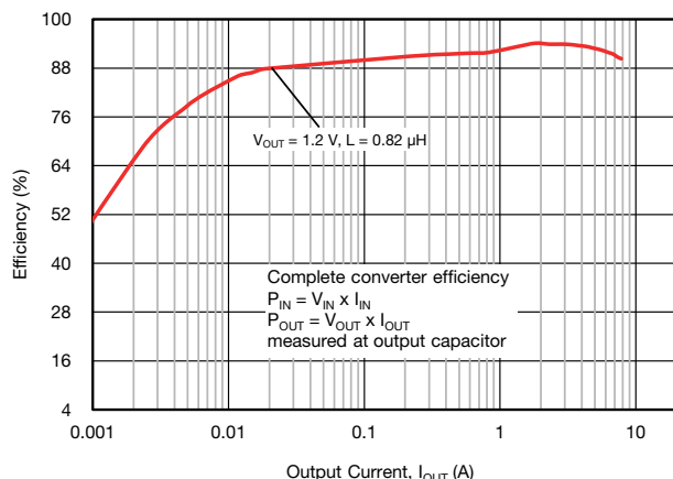
Fig. 18 - SiC438 Efficiency vs. Output Current (V_{IN} = 5\text{ V}, f_{SW} = 500\text{ kHz}, \text{Power Saving Mode})
