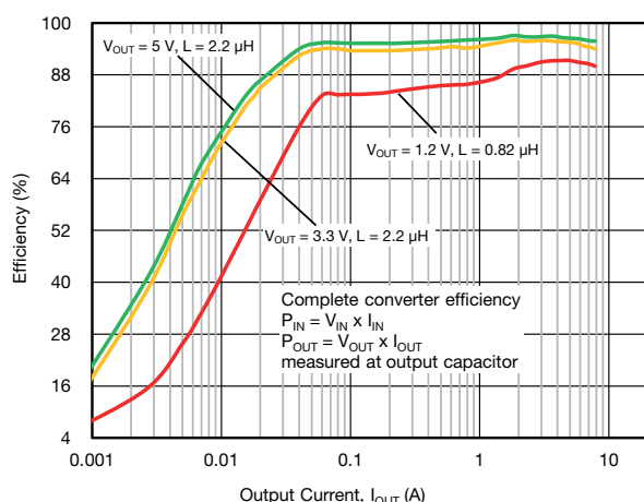
Fig. 17 - SiC438 Efficiency vs. Output Current (V_{IN} = 12\text{ V}, f_{SW} = 500\text{ kHz}, \text{Ultra Sonic Mode})
