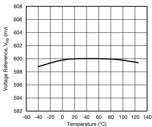
Fig. 23 - Voltage reference vs. Junction Temperature
