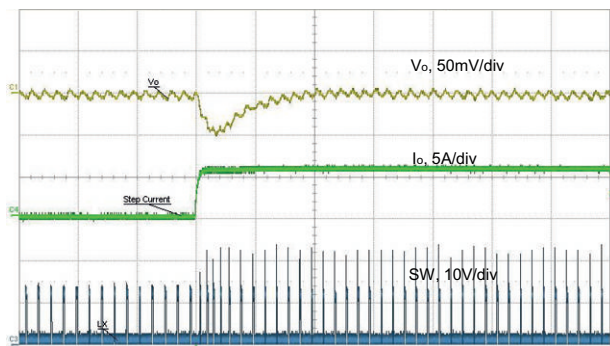
Fig. 39 - Load Step, 0.1 A to 6 A, 1 A/ \mu s, t = 10\text{ }\mu\text{s/div} Forced Continuous Conduction Mode
