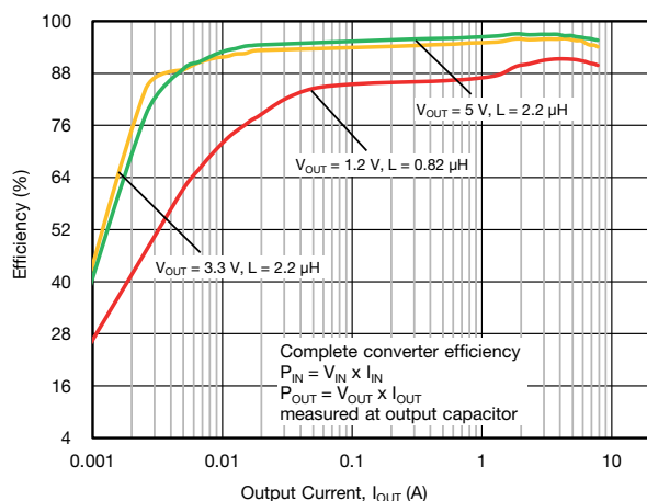
Fig. 16 - SiC438 Efficiency vs. Output Current (V_{IN} = 12\text{ V}, f_{SW} = 500\text{ kHz}, \text{Power Saving Mode})
