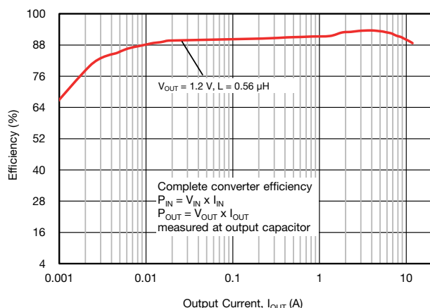
Fig. 12 - SiC437 Efficiency vs. Output Current (V_{IN} = 5\text{ V}, f_{SW} = 500\text{ kHz}, \text{Power Saving Mode})
