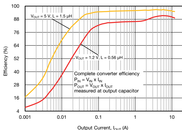
Fig. 11 - SiC437 Efficiency vs. Output Current (V_{IN} = 12\text{ V}, f_{SW} = 500\text{ kHz}, \text{Ultra Sonic Mode})
