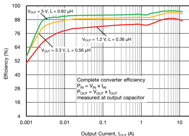
Fig. 13 - SiC437 Efficiency vs. Output Current (V_{IN} = 12\text{ V}, f_{SW} = 1\text{ MHz}, \text{Power Saving Mode})
