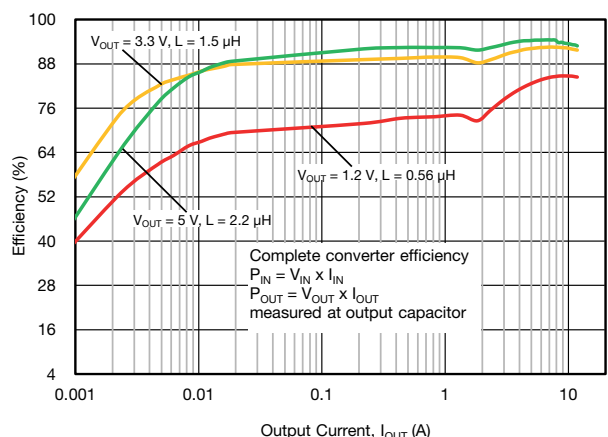
Fig. 15 - SiC437 Efficiency vs. Output Current (V_{IN} = 24\text{ V}, f_{SW} = 500\text{ kHz}, \text{Power Saving Mode})
