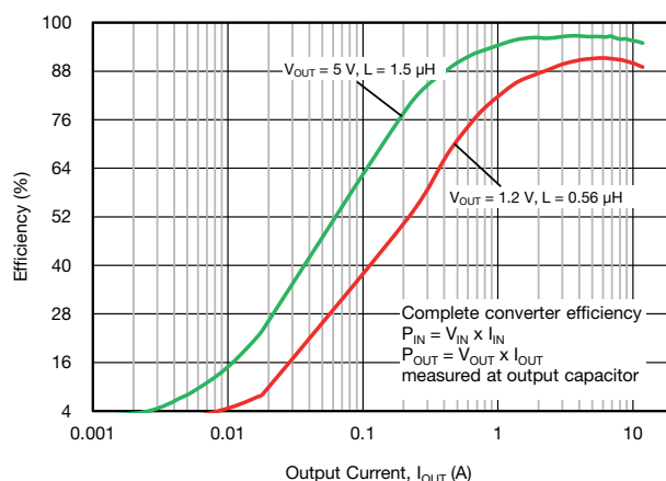
Fig. 14 - SiC437 Efficiency vs. Output Current (V_{IN} = 12\text{ V}, f_{SW} = 500\text{ kHz}, \text{Continuous Conduction Mode})
