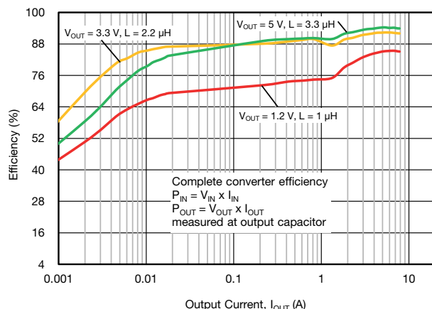
Fig. 21 - SiC438 Efficiency vs. Output Current (V_{IN} = 24\text{ V}, f_{SW} = 500\text{ kHz}, \text{Power Saving Mode})
