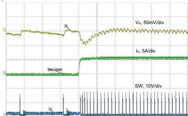
Fig. 38 - Load Step, 0.1 A to 6 A, 1 A/ \mu s, t = 10\text{ }\mu\text{s/div} Skip Mode Enabled
