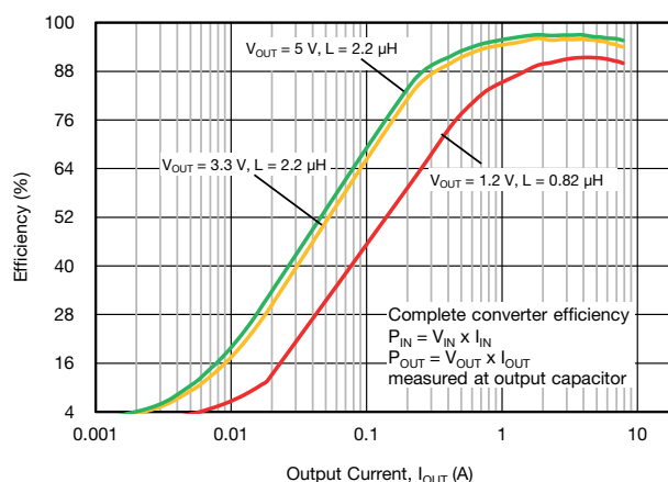
Fig. 20 - SiC438 Efficiency vs. Output Current (V_{IN} = 12\text{ V}, f_{SW} = 500\text{ kHz}, \text{Continuous Conduction Mode})
