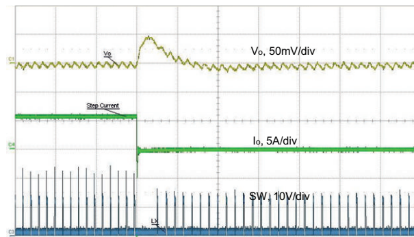
Fig. 42 - Load Release, 6 A to 0.1 A, 1 A/ \mu s, t = 10\text{ }\mu\text{s/div} Forced Continuous Conduction Mode
