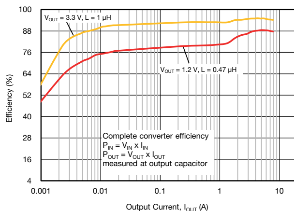
Fig. 19 - SiC438 Efficiency vs. Output Current (V_{IN} = 12\text{ V}, f_{SW} = 1\text{ MHz}, \text{Power Saving Mode})
