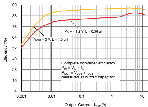
Fig. 2 - Efficiency vs. Output Current (V_{IN} = 12\text{ V}, f_{sw} = 500\text{ kHz}, \text{Power Saving Mode})
