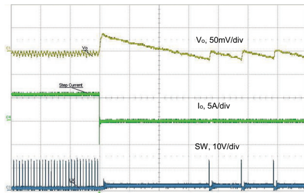
Fig. 41 - Load Release, 6 A to 0.1 A, 1 A/ \mu s, t = 20\text{ }\mu\text{s/div} Skip Mode Enabled
