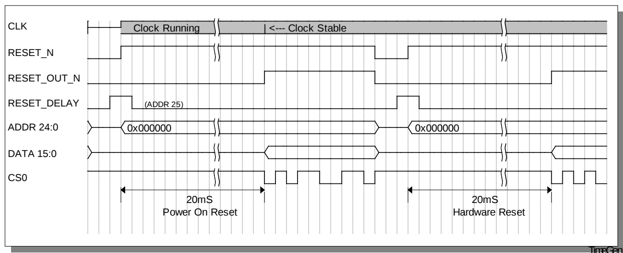
Figure 8. Extended Reset Timing
