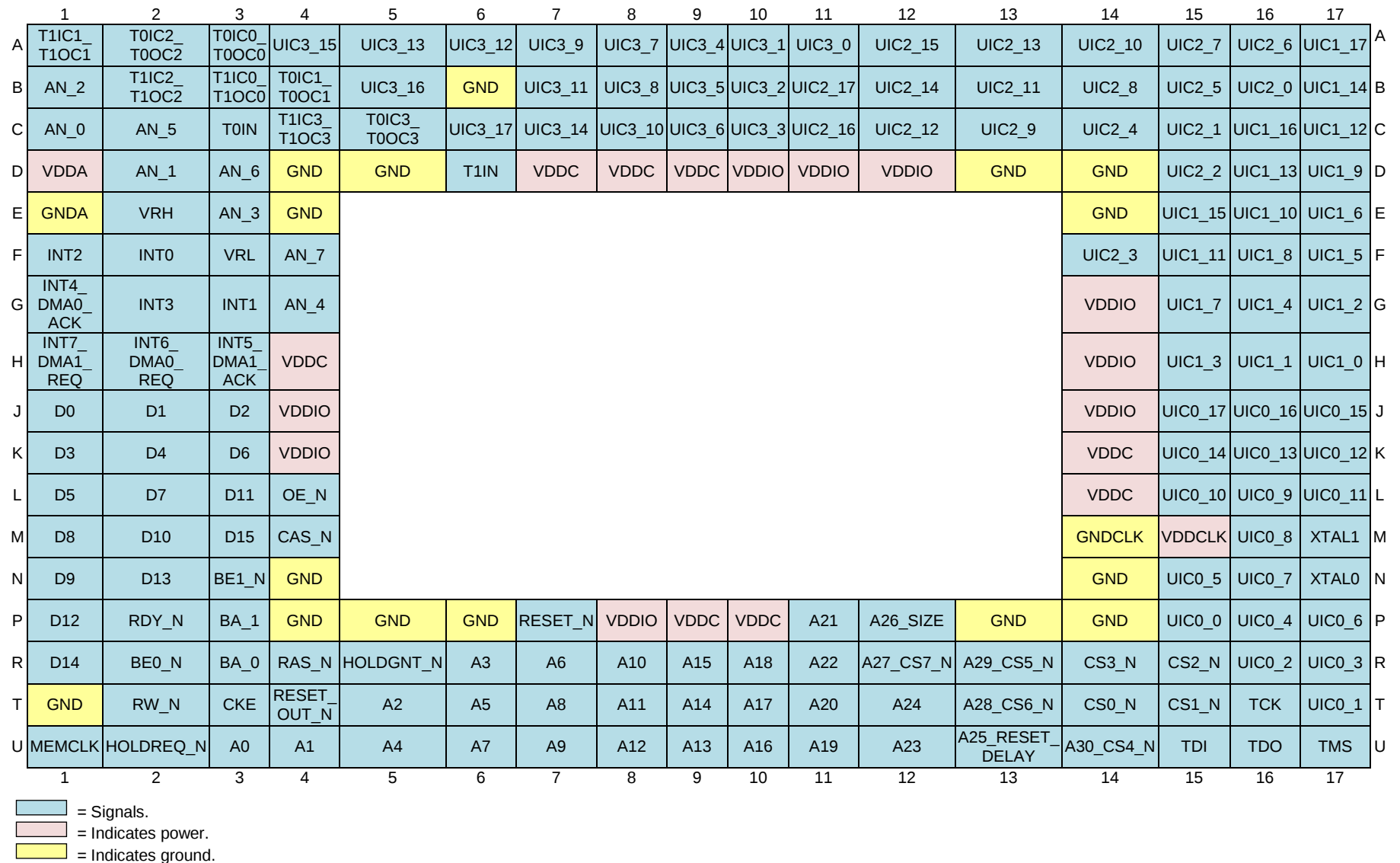
Figure 4. BGA 15- by 15-mm Package Diagram
